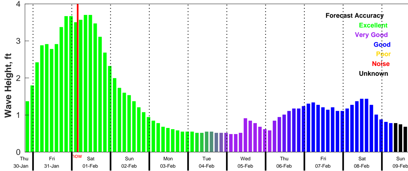
CMEMS Wave Forecast for NDBC 42036 from 30-Jan-2025 19:00:00 to 09-Feb-2025 19:00:00
