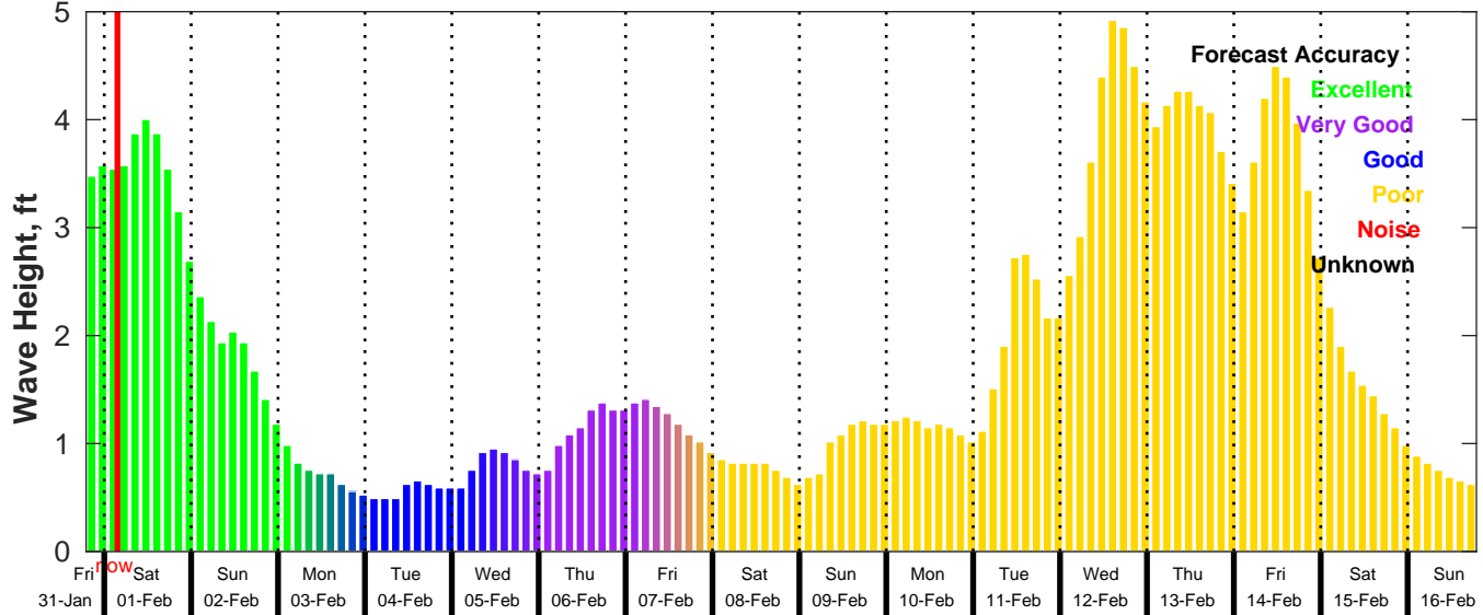
GFS Wave Forecast for NDBC 42036 from 31-Jan-2025 19:00:00 to 16-Feb-2025 19:00:00
