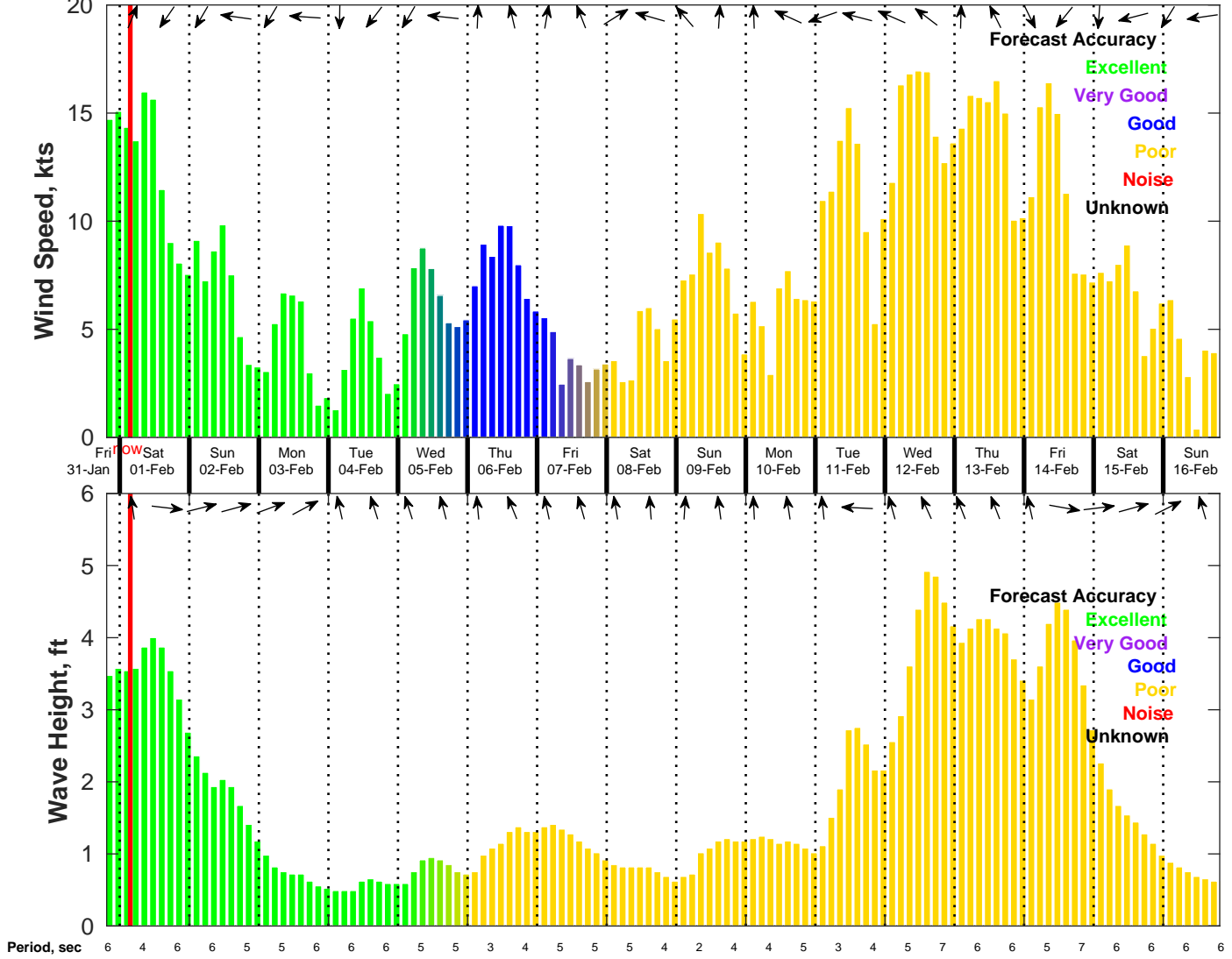
Wind & Wave Forecast for NDBC 42036 from 31-Jan-2025 19:00:00 to 16-Feb-2025 19:00:00
