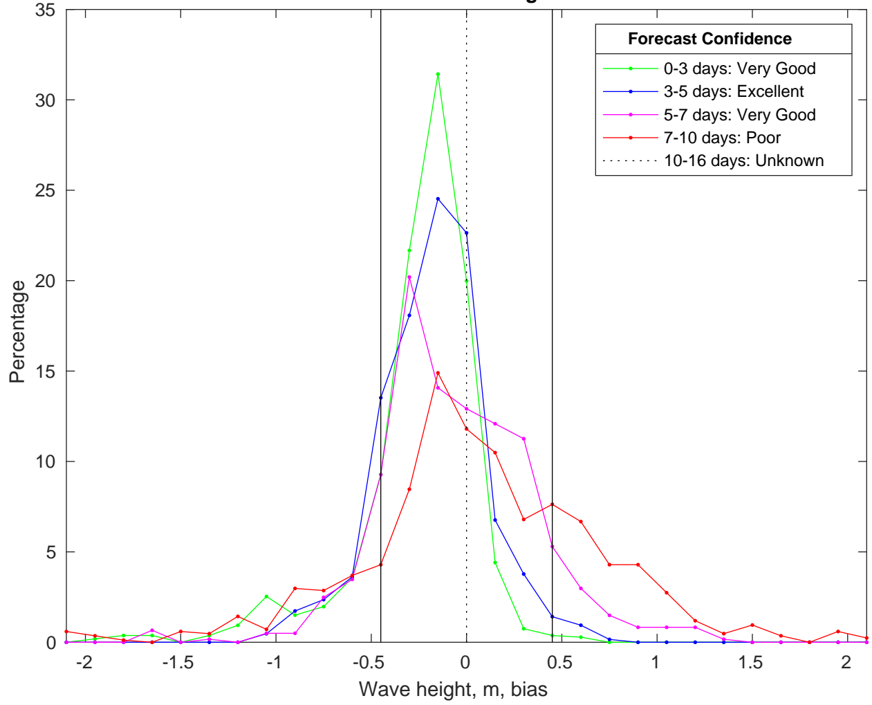
NDBC 42040 vs CMEMSWaves Bias Histogram: 01-Feb-2025
