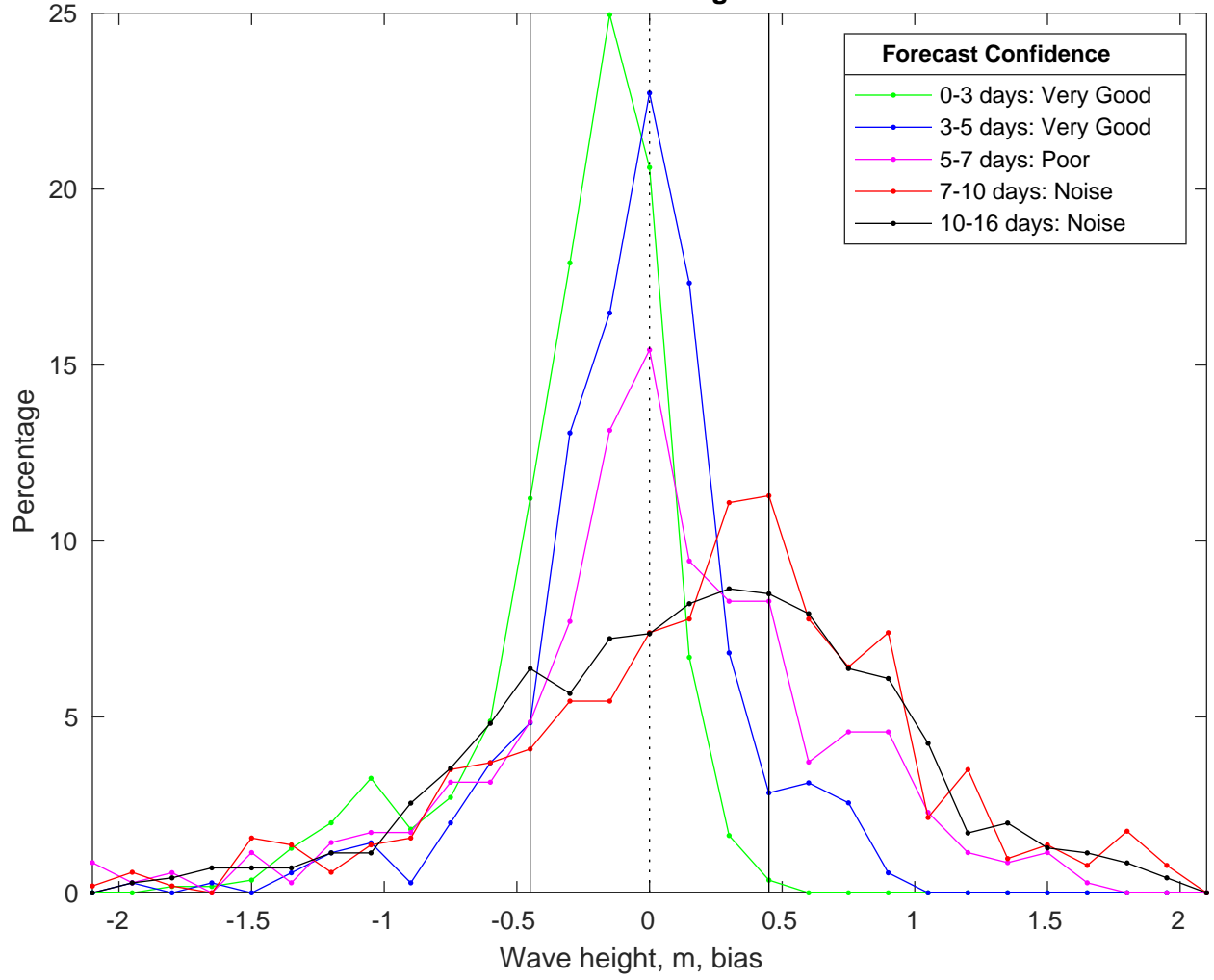
NDBC 42040 vs GFSWaves Bias Histogram: 01-Feb-2025
