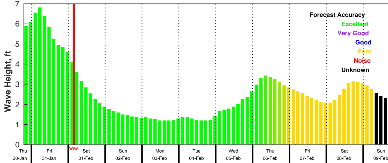
CMEMS Wave Forecast for NDBC 42084 from 30-Jan-2025 19:00:00 to 09-Feb-2025 19:00:00
