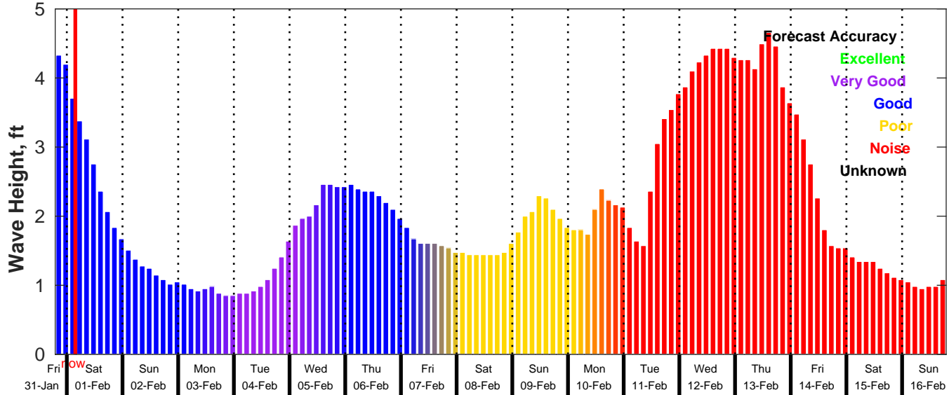
GFS Wave Forecast for NDBC 42084 from 31-Jan-2025 19:00:00 to 16-Feb-2025 19:00:00
