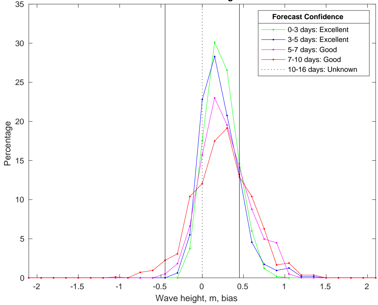
NDBC 44020 vs CMEMSWaves Bias Histogram: 01-Feb-2025
