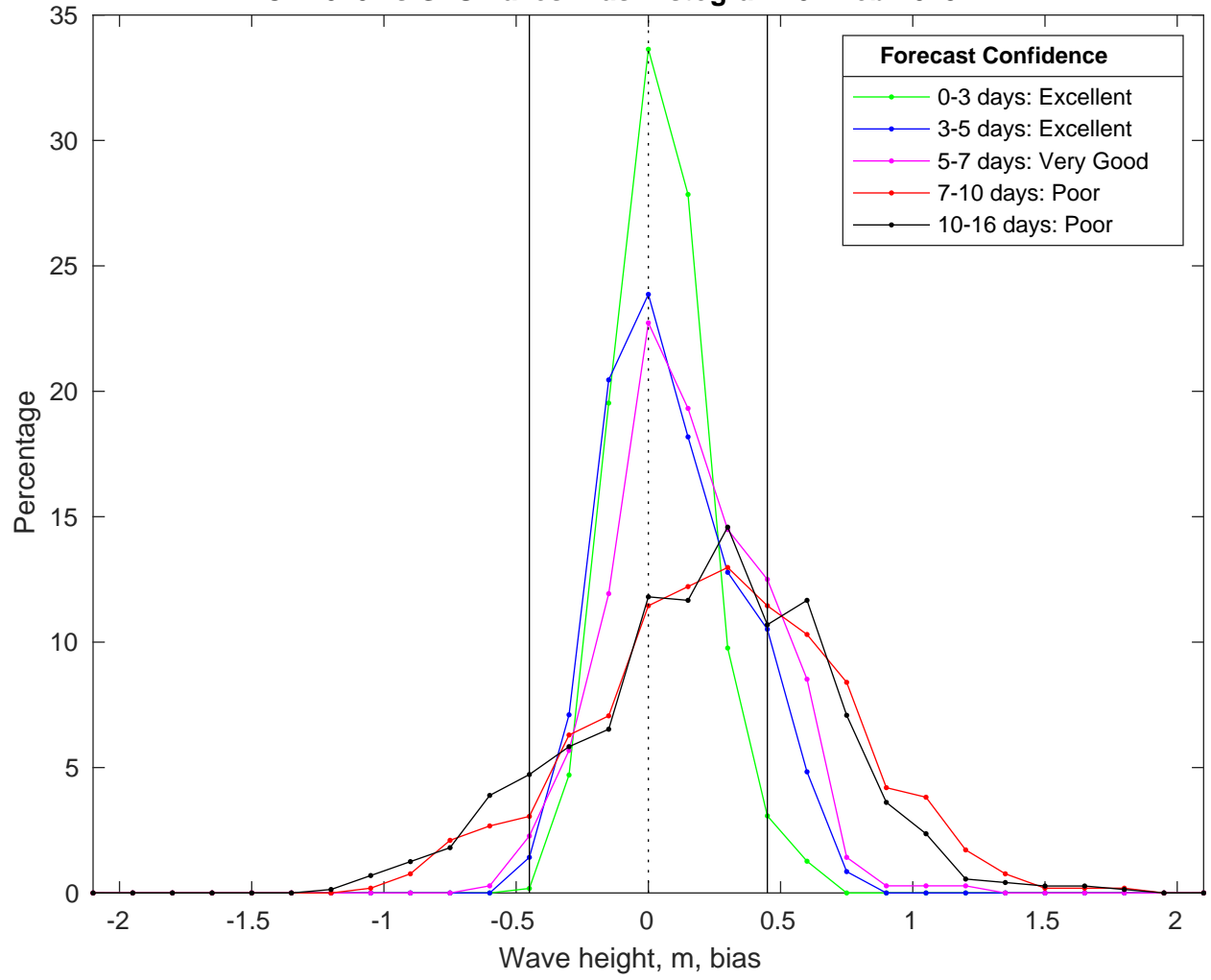
NDBC 44020 vs GFSWaves Bias Histogram: 01-Feb-2025
