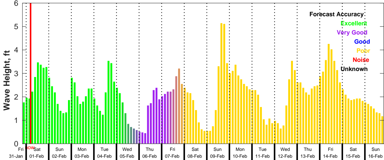
GFS Wave Forecast for NDBC 44020 from 31-Jan-2025 20:00:00 to 16-Feb-2025 20:00:00
