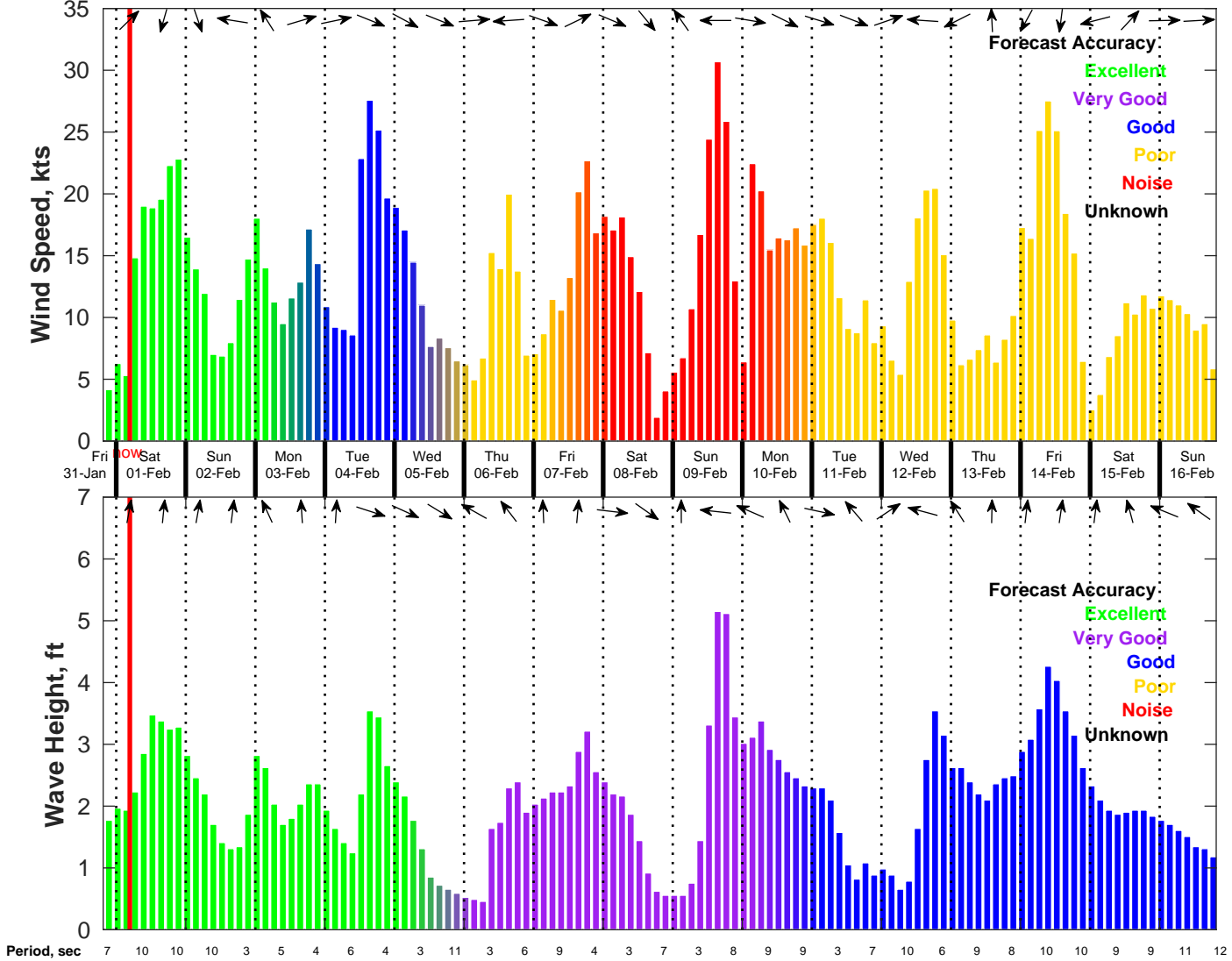
Wind & Wave Forecast for NDBC 44020 from 31-Jan-2025 20:00:00 to 16-Feb-2025 20:00:00
