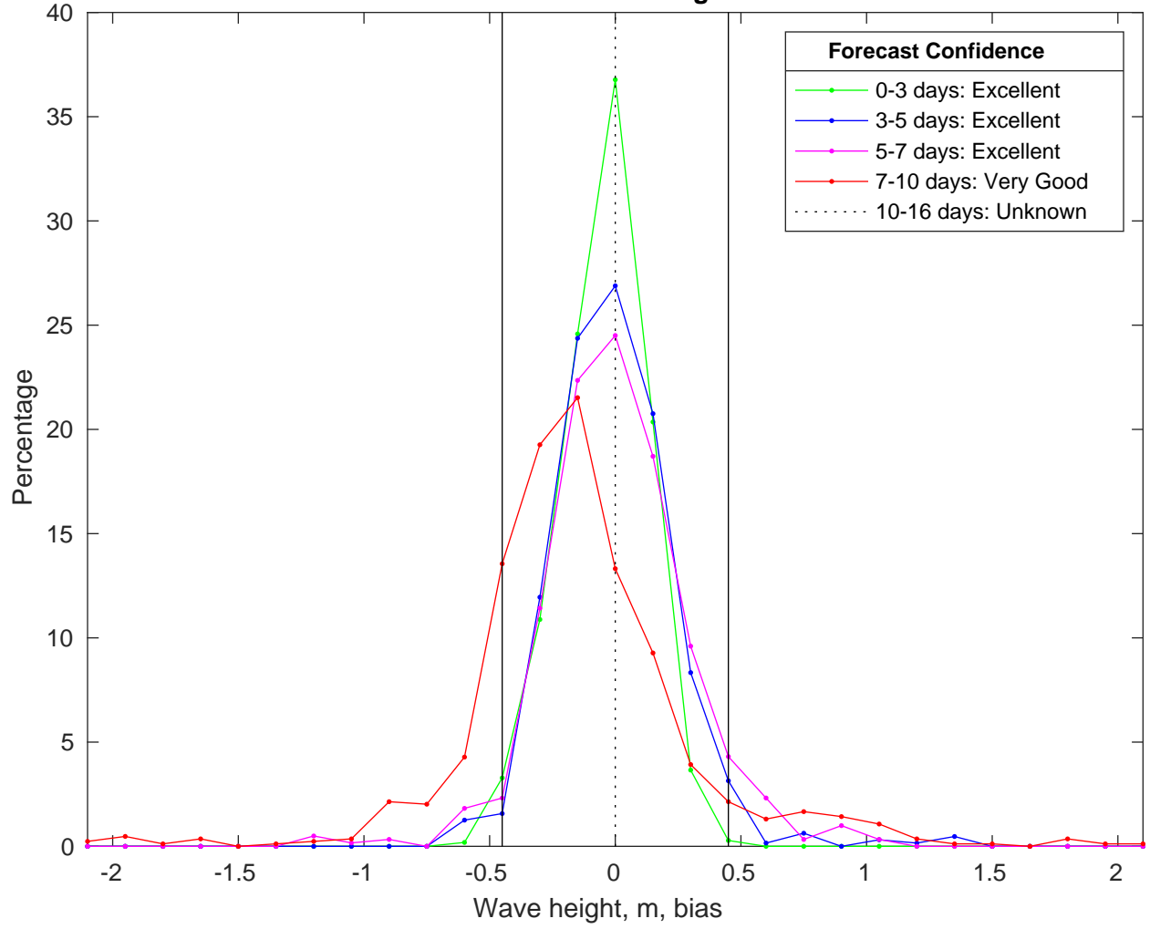
NDBC 46011 vs CMEMSWaves Bias Histogram: 01-Feb-2025
