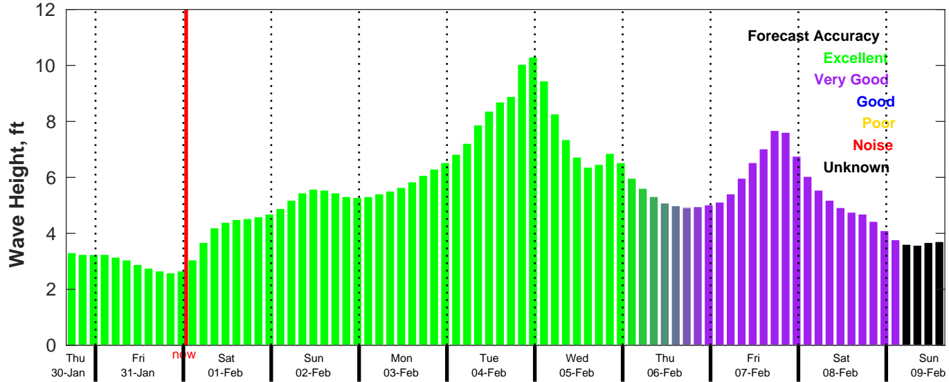
CMEMS Wave Forecast for NDBC 46011 from 30-Jan-2025 16:00:00 to 09-Feb-2025 16:00:00
