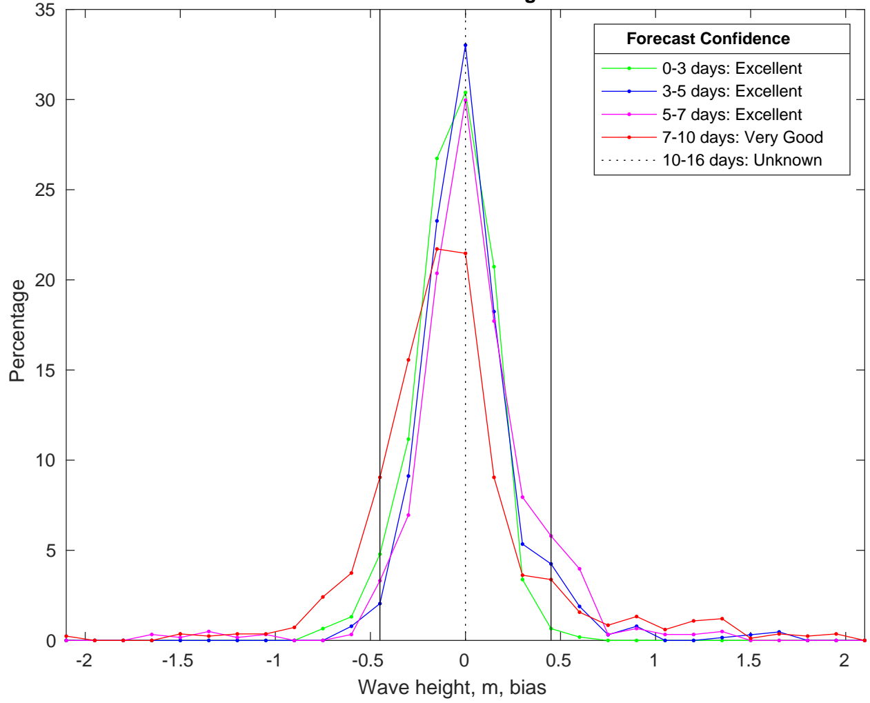
NDBC 46028 vs CMEMSWaves Bias Histogram: 01-Feb-2025
