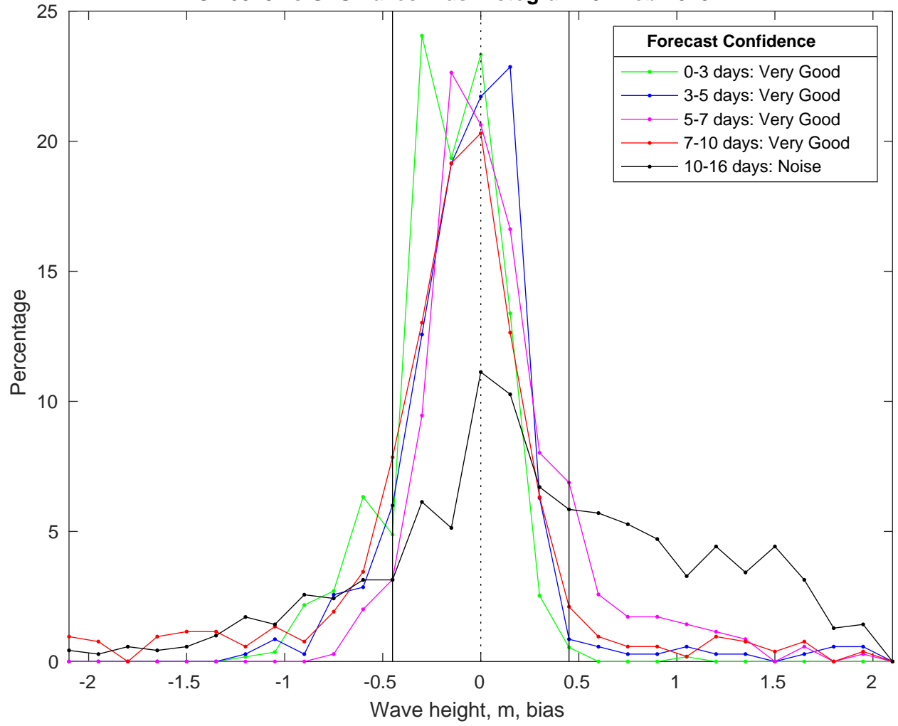
NDBC 46028 vs GFSWaves Bias Histogram: 01-Feb-2025
