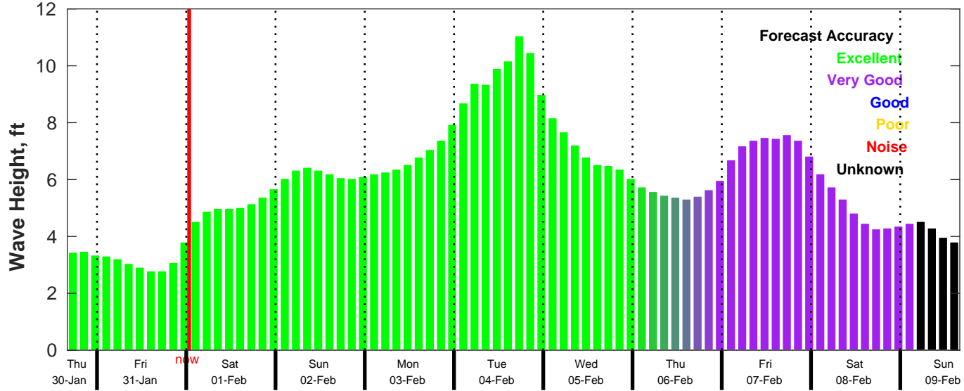
CMEMS Wave Forecast for NDBC 46028 from 30-Jan-2025 16:00:00 to 09-Feb-2025 16:00:00
