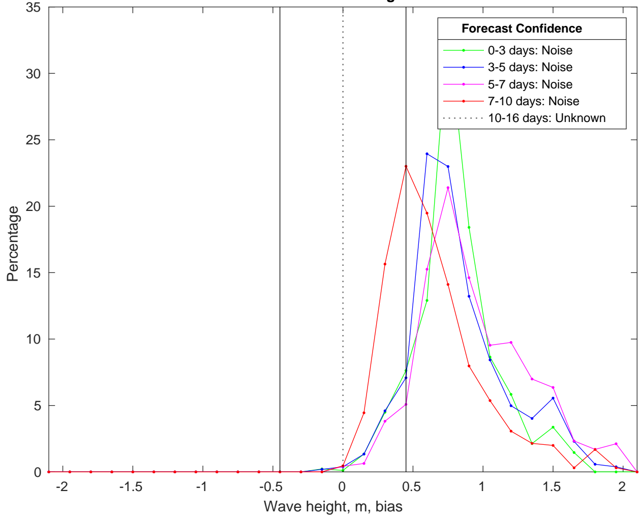
NDBC 46053 vs CEMSWaves Bias Histogram: 01-Feb-2025
