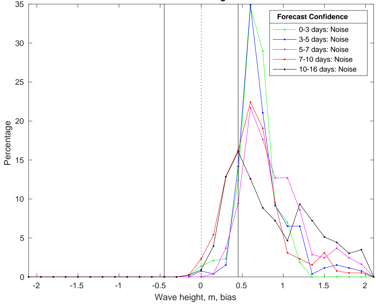
NDBC 46053 vs GFSWaves Bias Histogram: 01-Feb-2025
