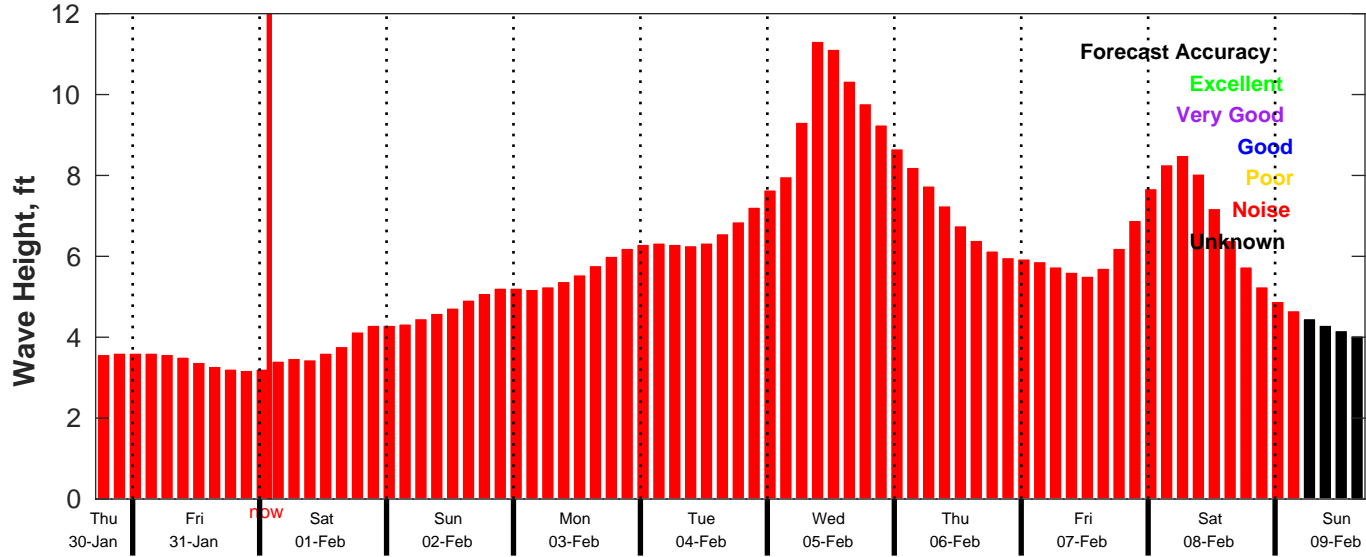
CMEMS Wave Forecast for NDBC 46053 from 30-Jan-2025 17:00:00 to 09-Feb-2025 17:00:00
