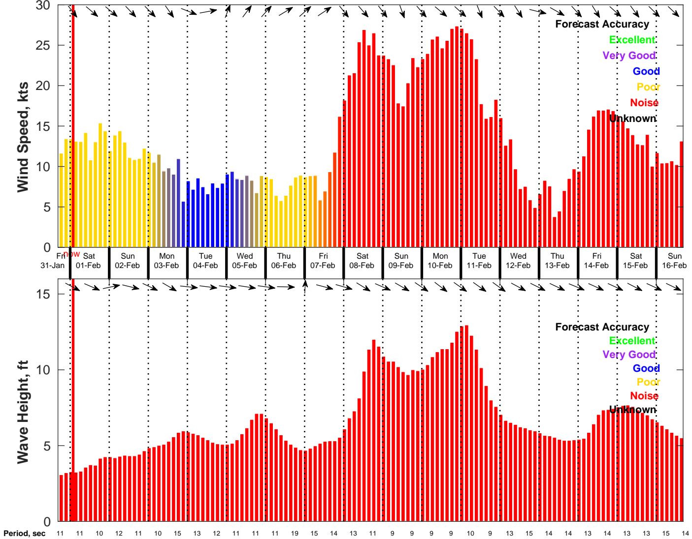
Wind & Wave Forecast for NDBC 46053 from 31-Jan-2025 17:00:00 to 16-Feb-2025 17:00:00
