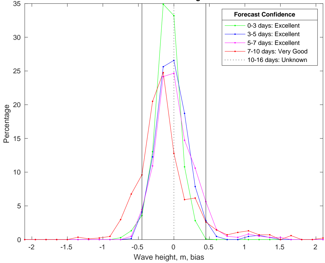
NDBC 46054 vs CMEMSWaves Bias Histogram: 01-Feb-2025
