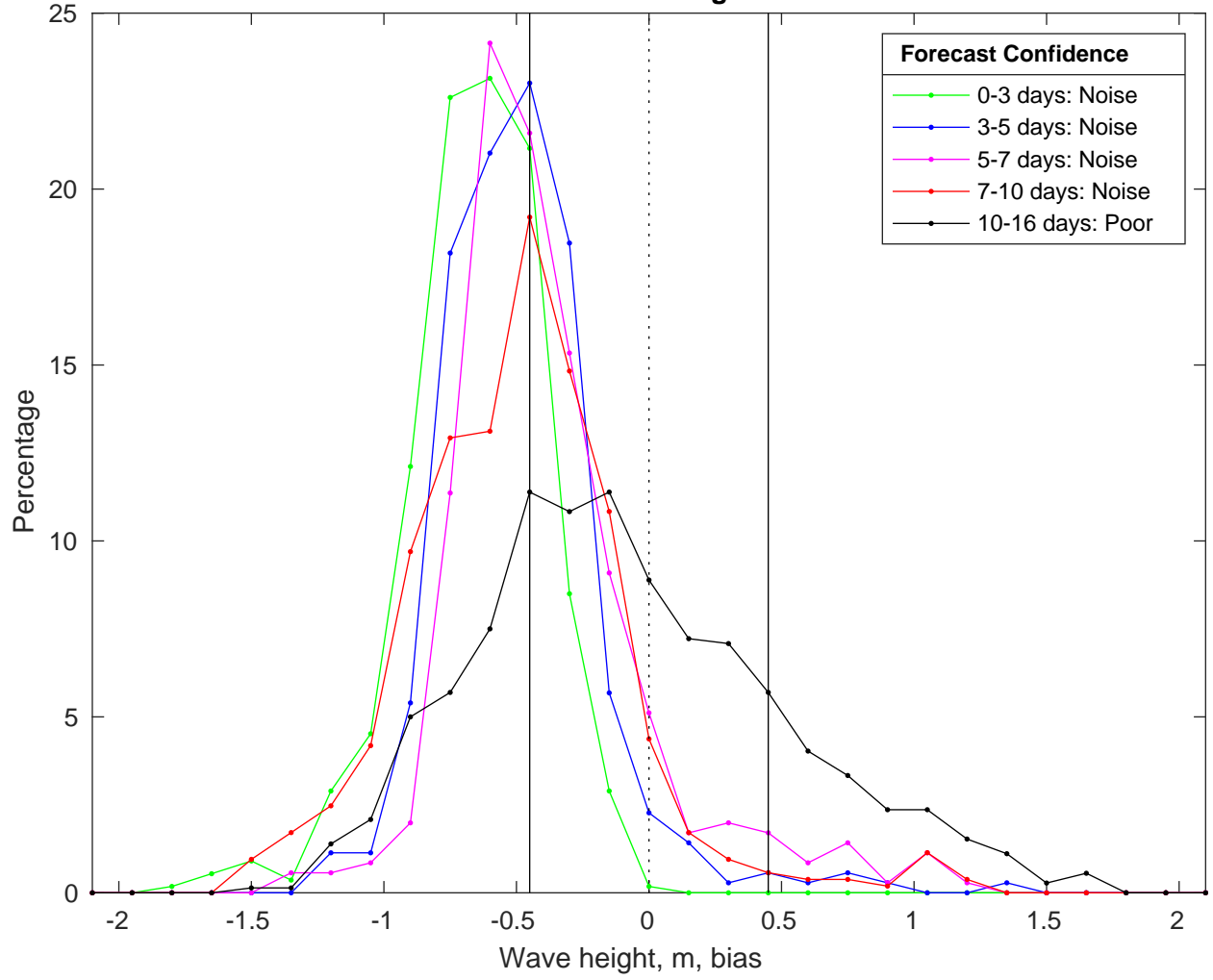
NDBC 46054 vs GFSWaves Bias Histogram: 01-Feb-2025
