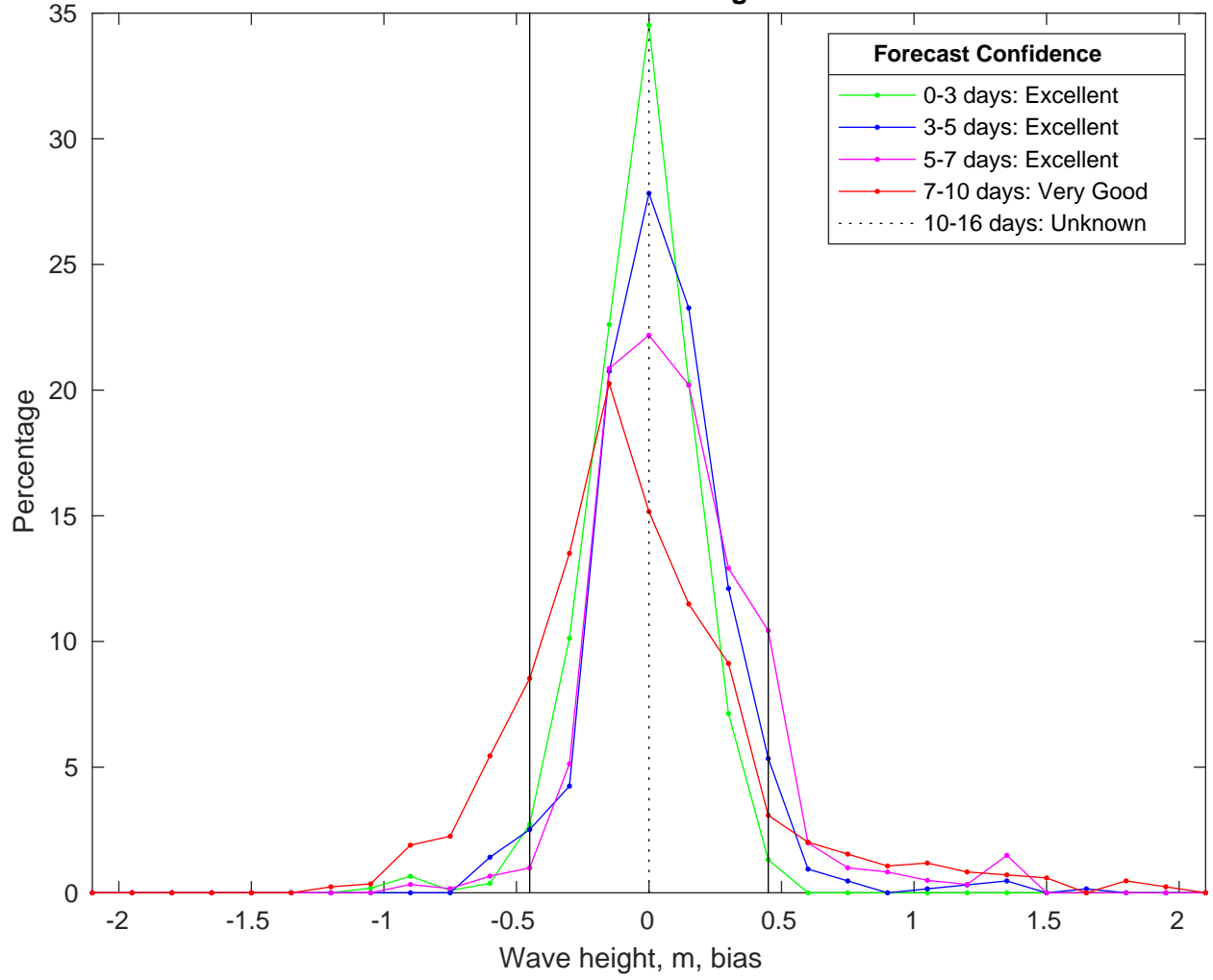
NDBC 46069 vs CMEMSWaves Bias Histogram: 01-Feb-2025
