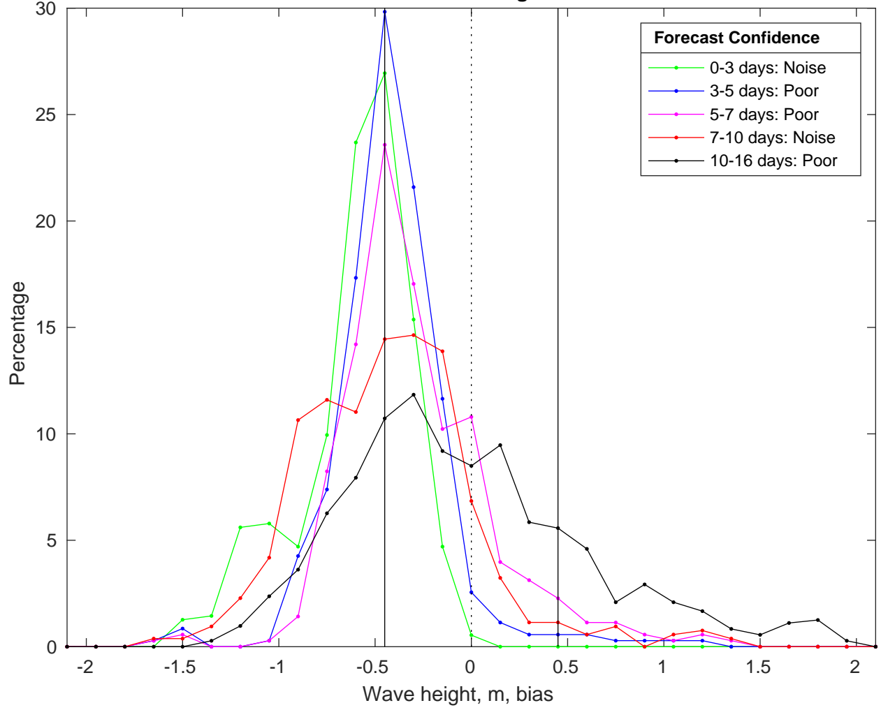
NDBC 46069 vs GFSWaves Bias Histogram: 01-Feb-2025
