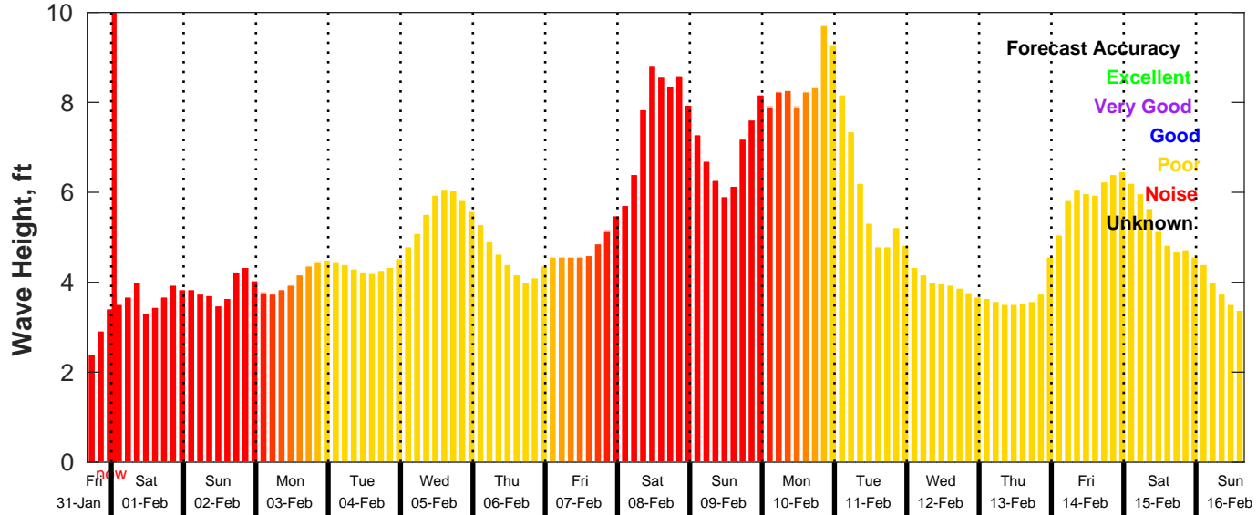
GFS Wave Forecast for NDBC 46069 from 31-Jan-2025 16:00:00 to 16-Feb-2025 16:00:00
