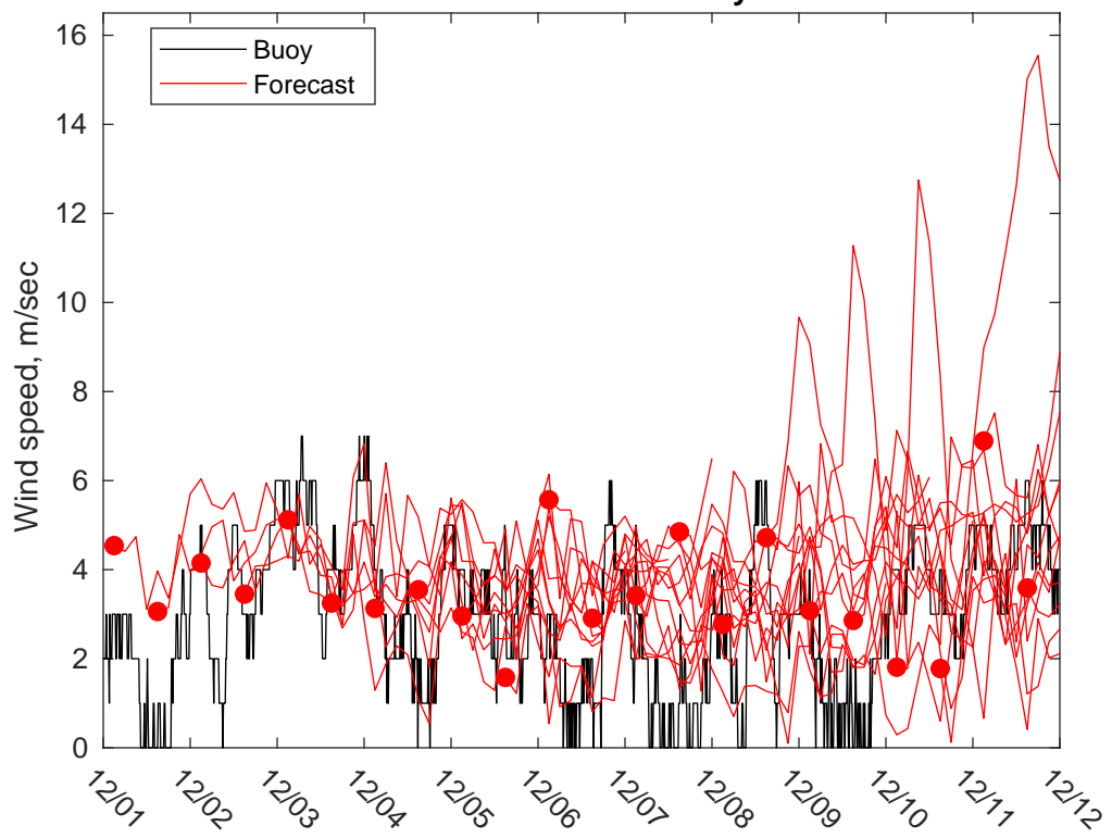
NDBC 46086 vs GFSWinds: 10 to 16 day forecast
