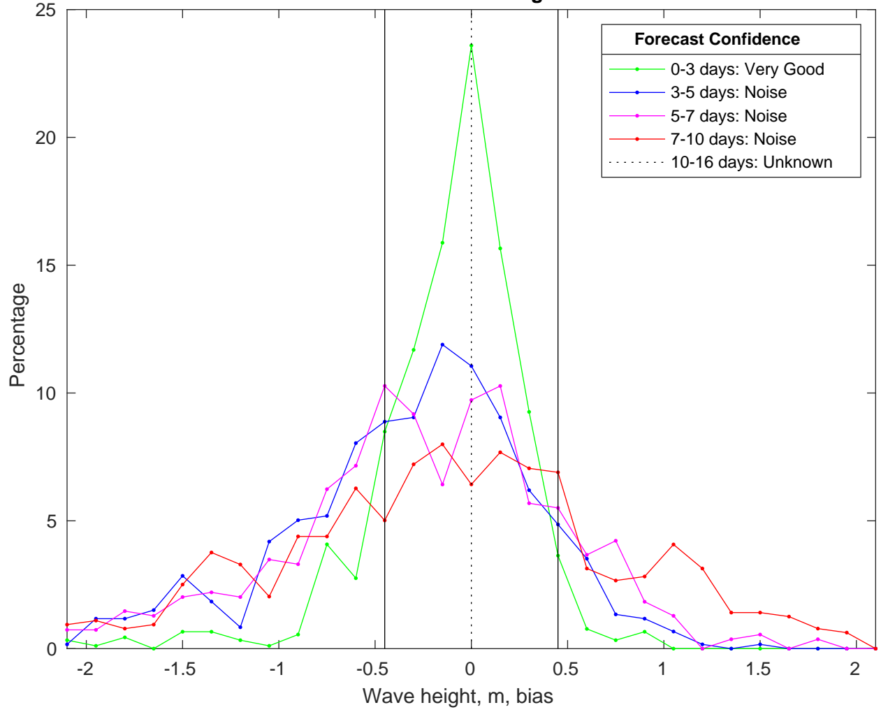
NDBC 46246 vs CMEMSWaves Bias Histogram: 01-Feb-2025
