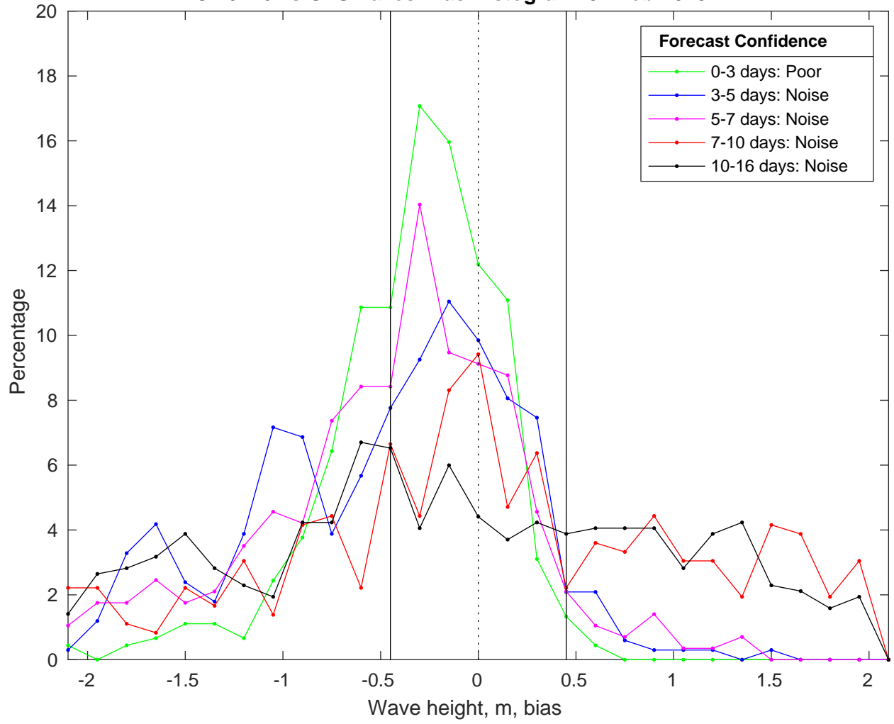
NDBC 46246 vs GFSWaves Bias Histogram: 01-Feb-2025
