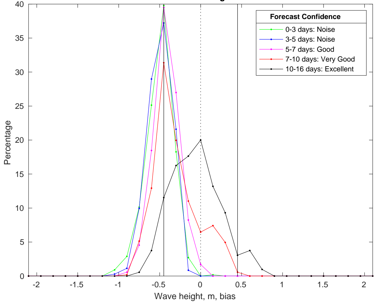
NDBC 51209 vs GFSWaves Bias Histogram: 01-Feb-2025
