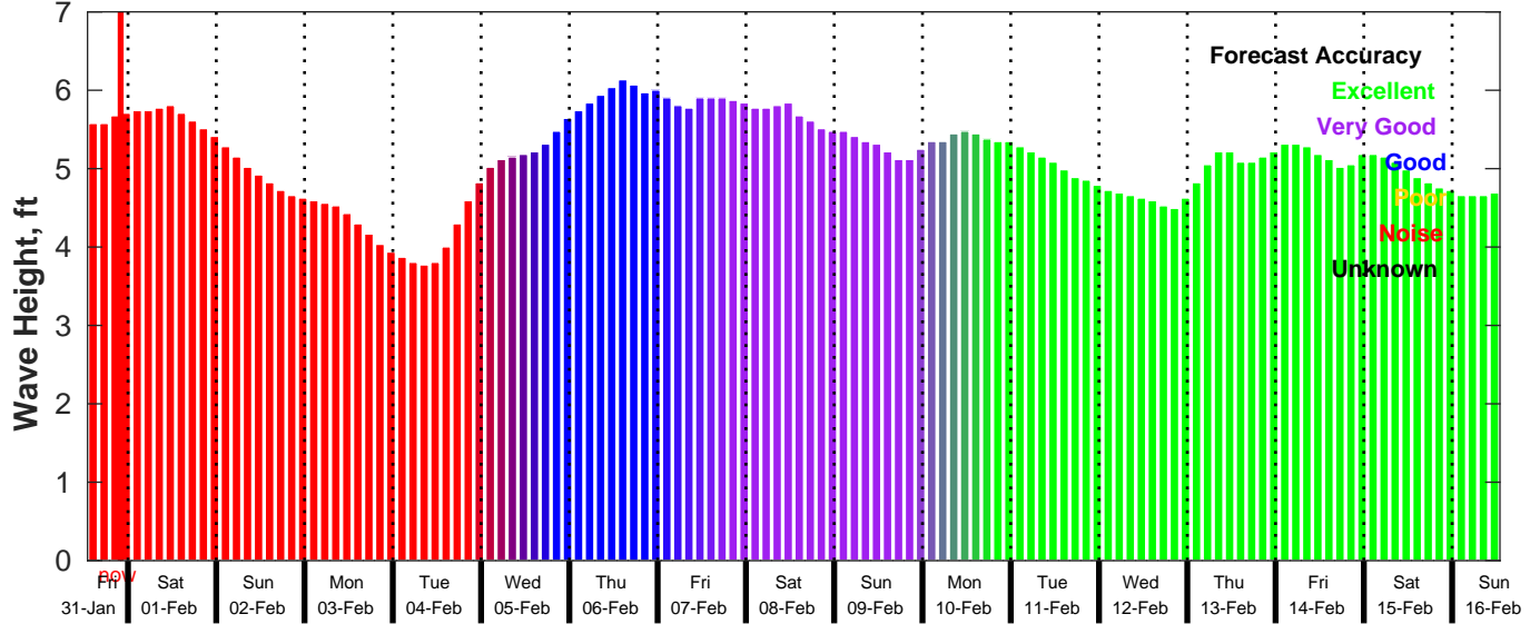
GFS Wave Forecast for NDBC 51209 from 31-Jan-2025 13:00:00 to 16-Feb-2025 13:00:00
