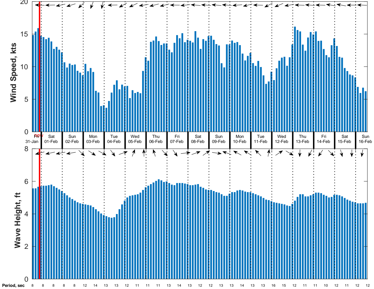
Wind & Wave Forecast for NDBC 51209 from 31-Jan-2025 13:00:00 to 16-Feb-2025 13:00:00
