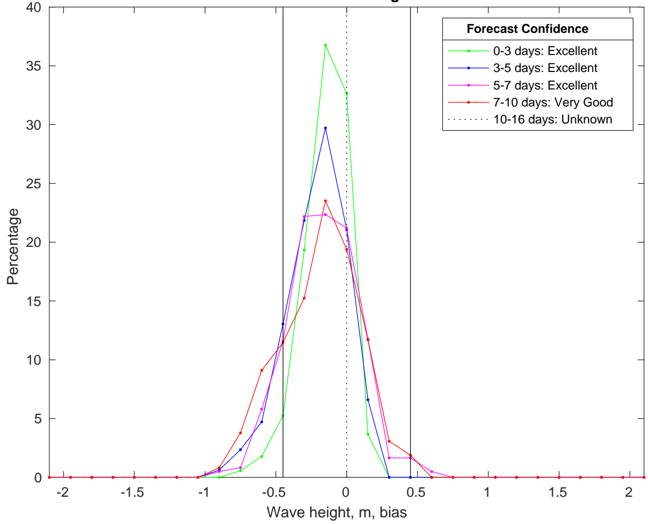
NDBC 52211 vs CMEMSWaves Bias Histogram: 01-Feb-2025
