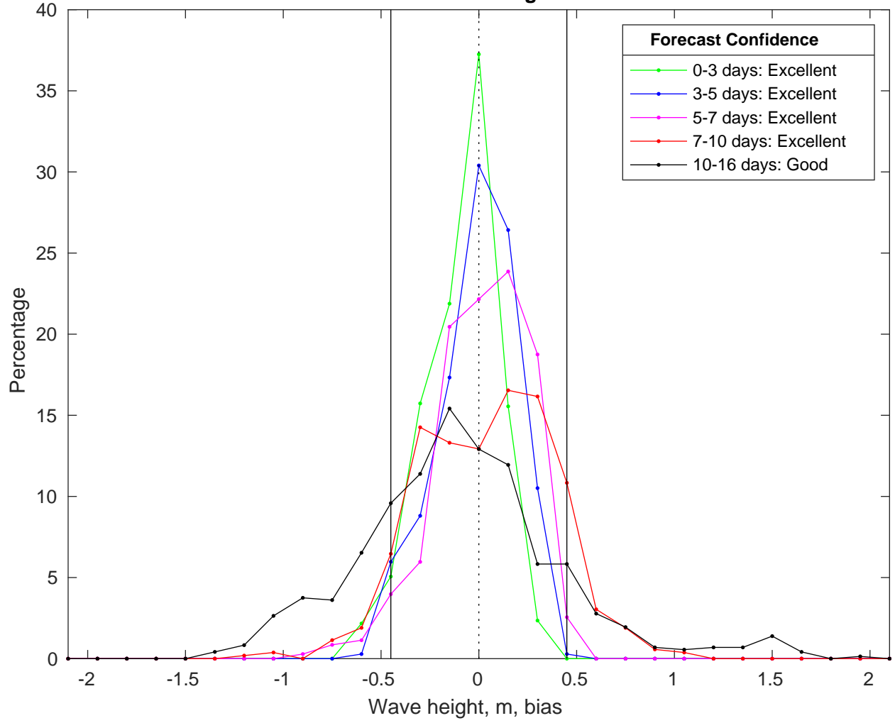
NDBC 52211 vs GFSWaves Bias Histogram: 01-Feb-2025
