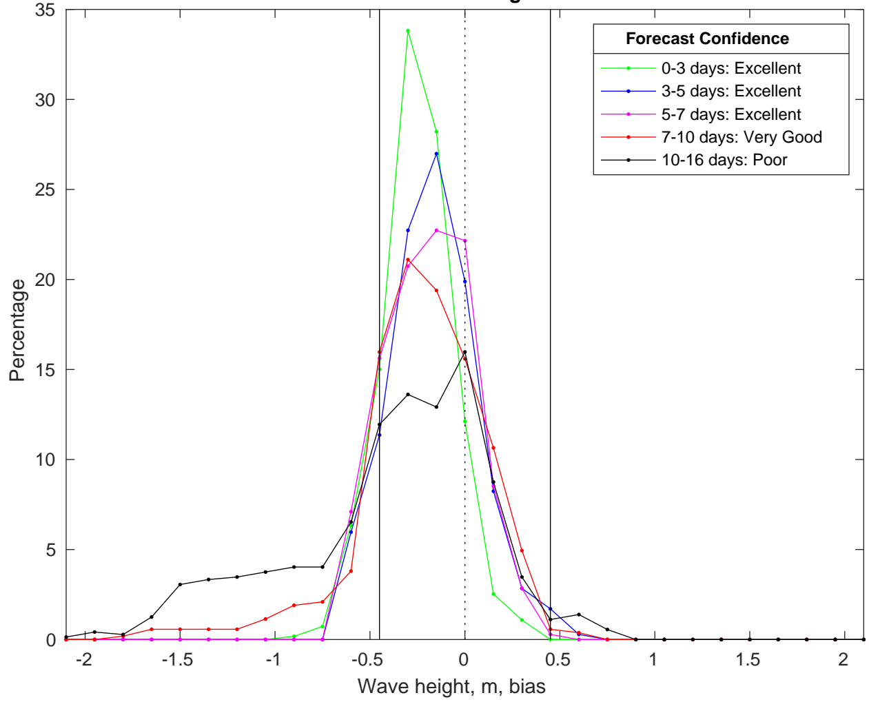
NDBC 52212 vs GFSWaves Bias Histogram: 01-Feb-2025
