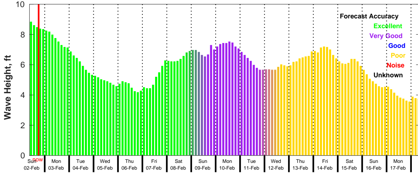
GFS Wave Forecast for NDBC 52212 from 01-Feb-2025 09:00:00 to 17-Feb-2025 09:00:00
