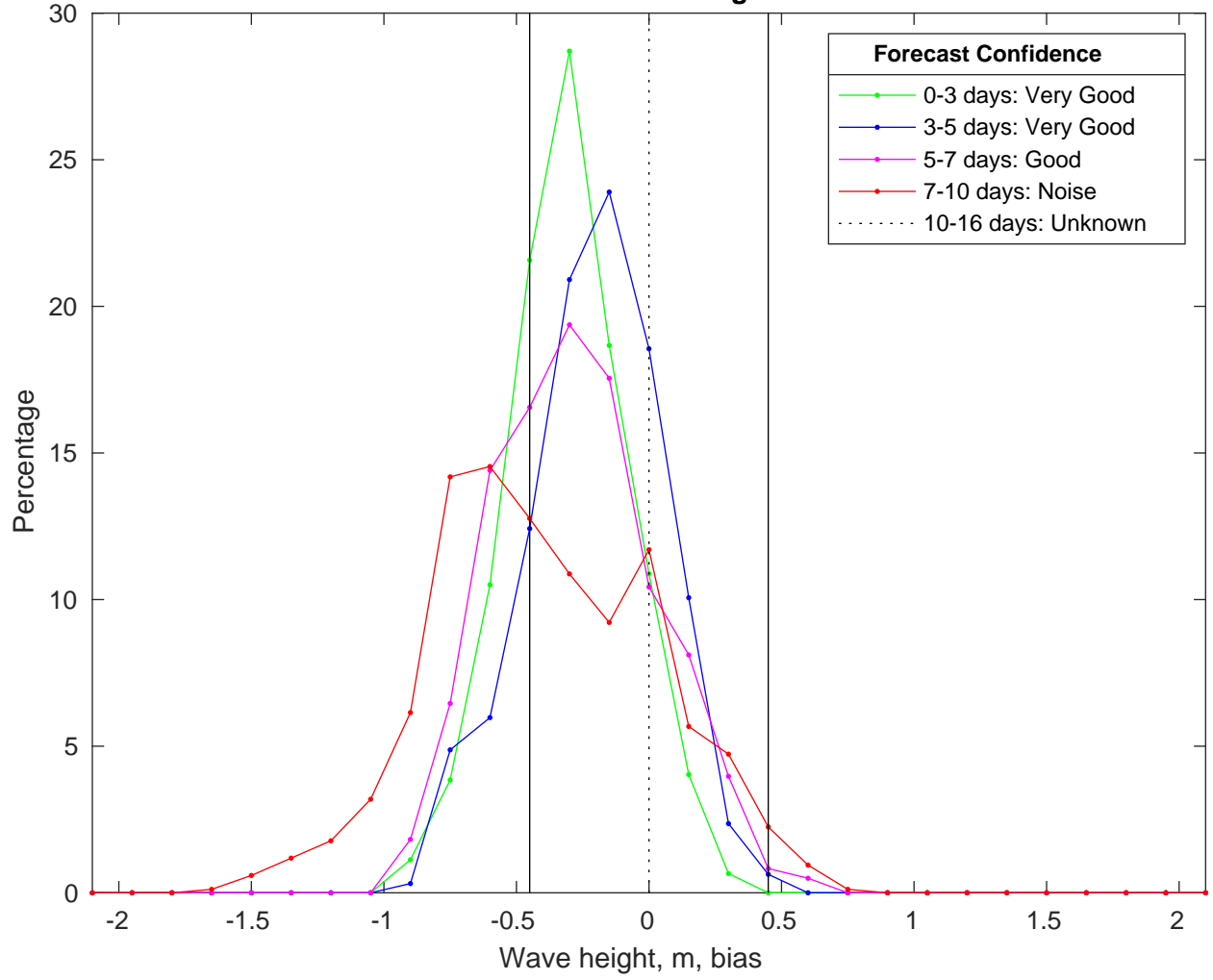
NDBC 52213 vs CMEMSWaves Bias Histogram: 01-Feb-2025
