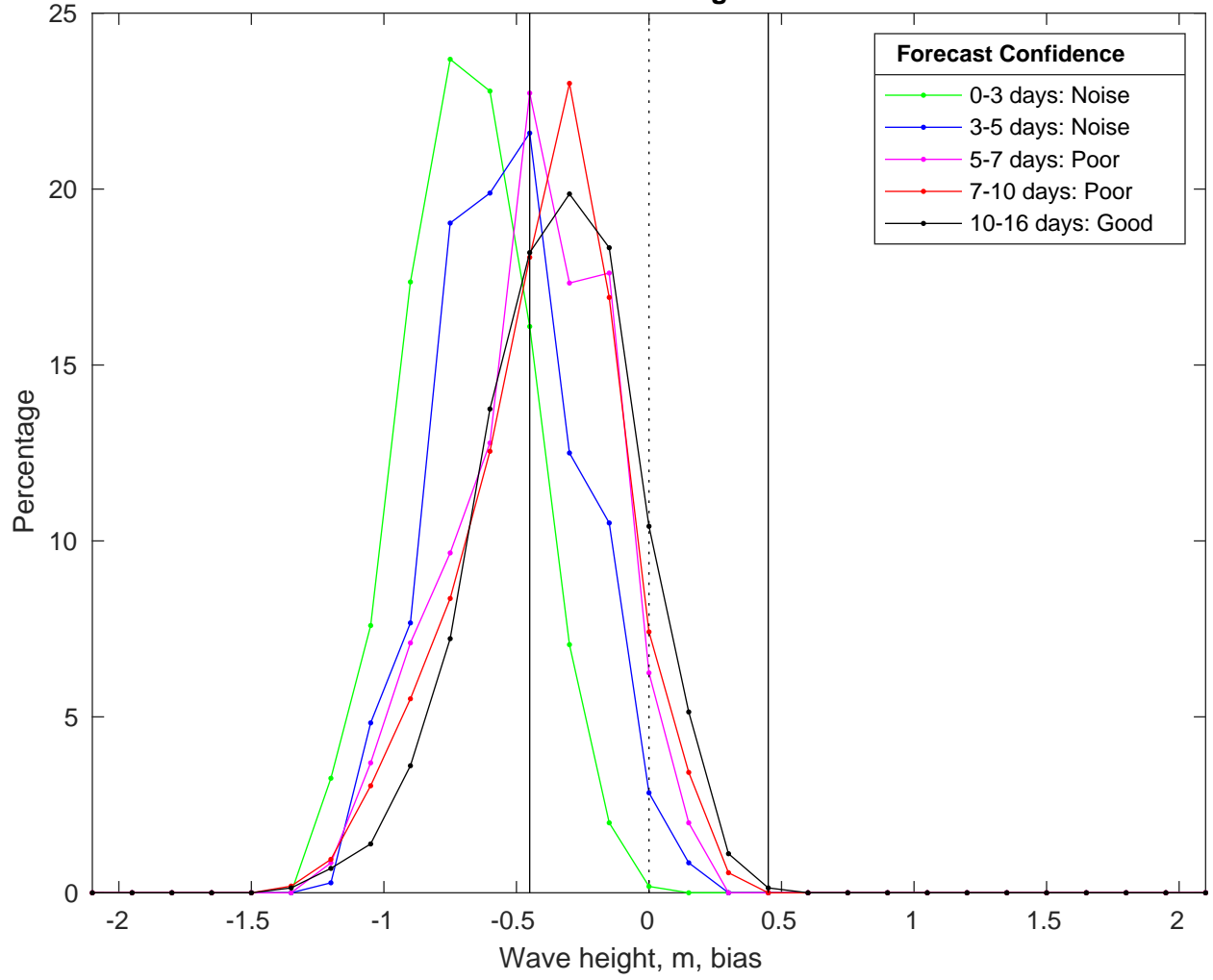
NDBC 52213 vs GFSWaves Bias Histogram: 01-Feb-2025
