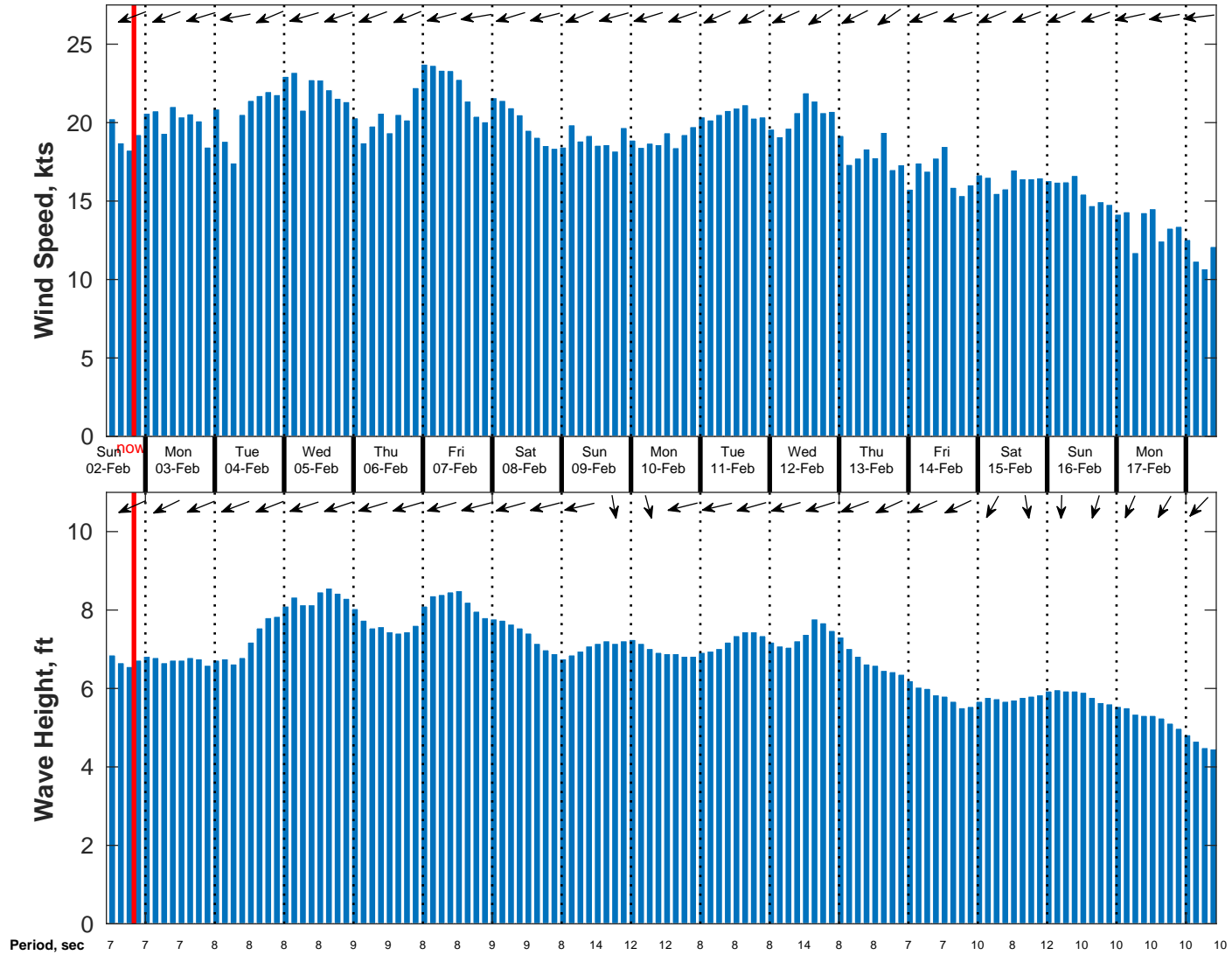
Wind & Wave Forecast for NDBC 52213 from 01-Feb-2025 11:00:00 to 17-Feb-2025 11:00:00
