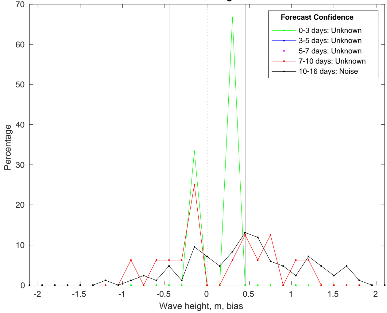
NDBC 62305 vs GFSWaves Bias Histogram: 01-Feb-2025
