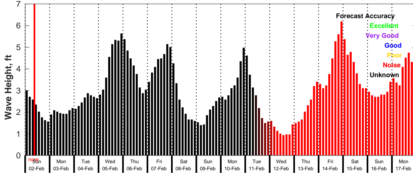
GFS Wave Forecast for NDBC 62305 from 01-Feb-2025 00:00:00 to 17-Feb-2025 00:00:00
