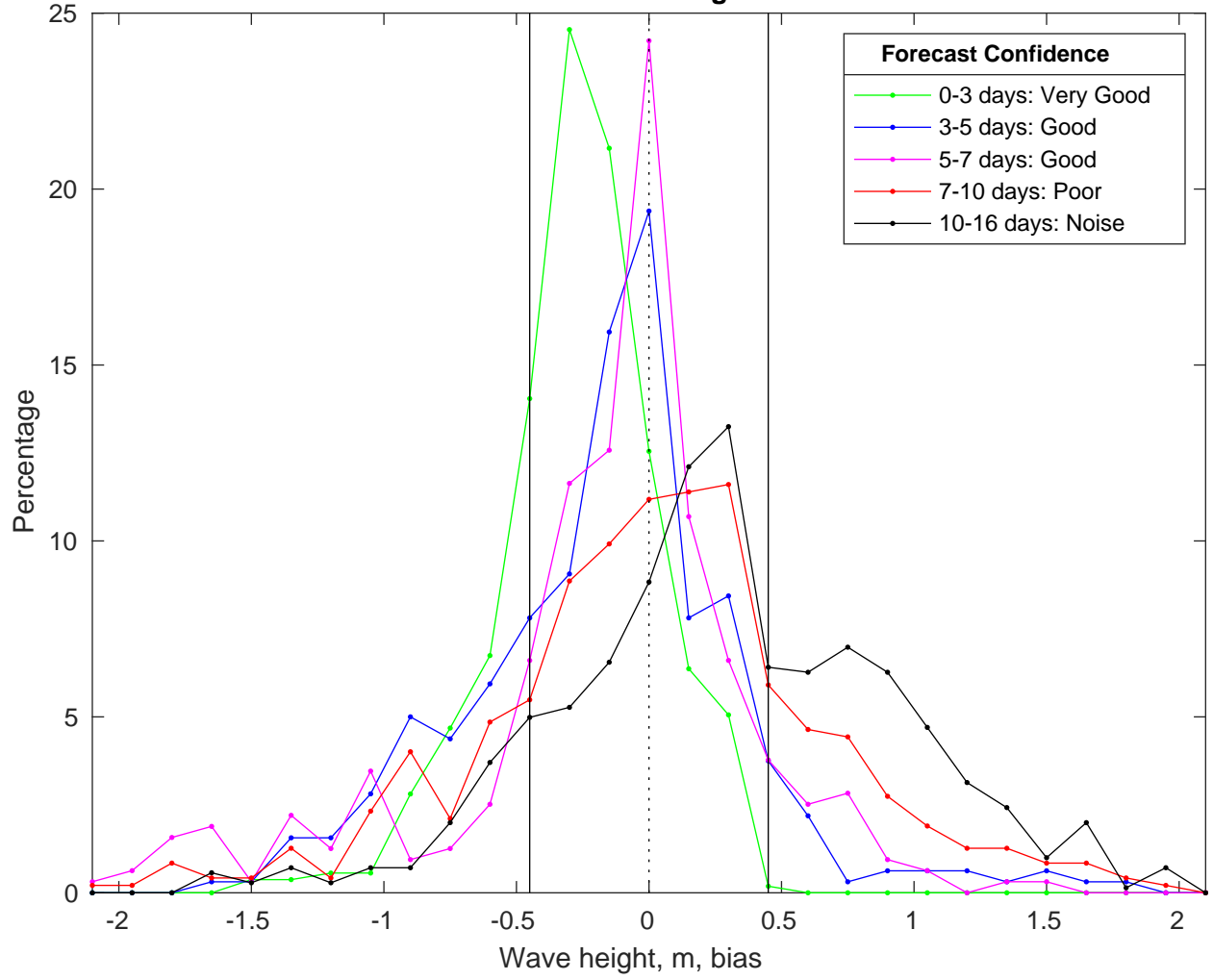
NDBC 41004 vs GFSWaves Bias Histogram: 02-Feb-2025
