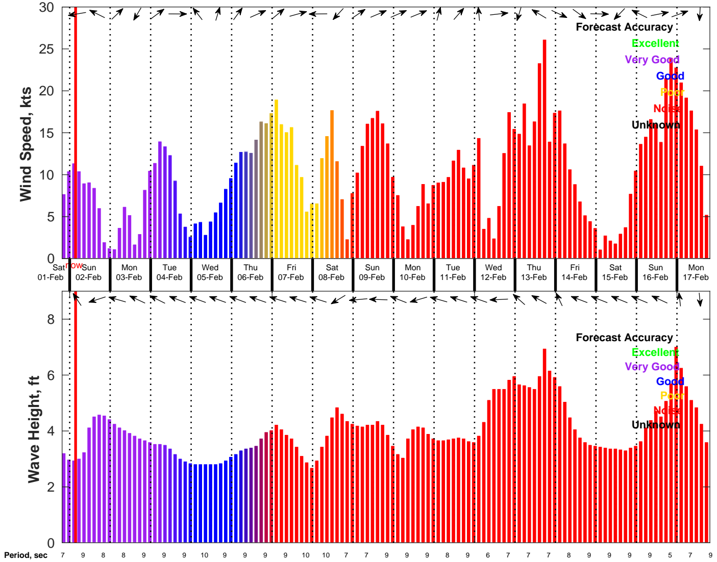
Wind & Wave Forecast for NDBC 41004 from 01-Feb-2025 19:00:00 to 17-Feb-2025 19:00:00
