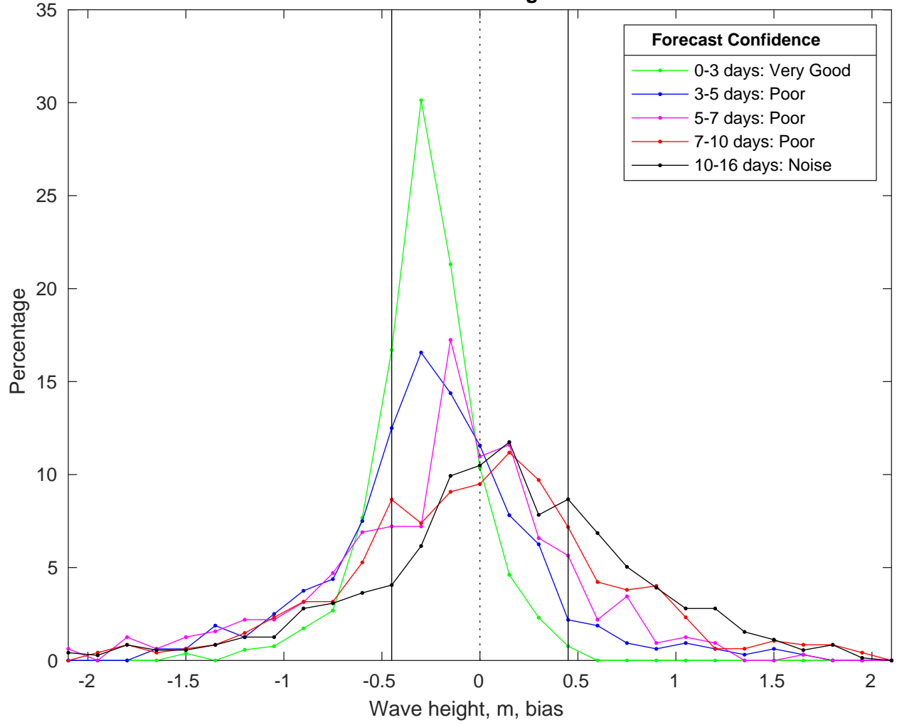
NDBC 41013 vs GFSWaves Bias Histogram: 02-Feb-2025
