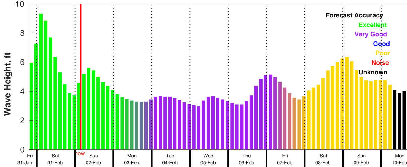
CMEMS Wave Forecast for NDBC 41013 from 31-Jan-2025 19:00:00 to 10-Feb-2025 19:00:00
