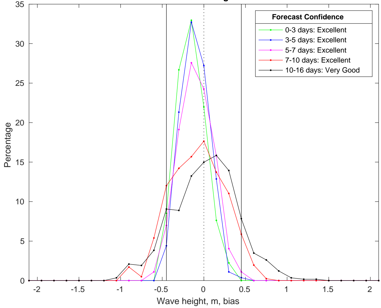
NDBC 41040 vs GFSWaves Bias Histogram: 02-Feb-2025
