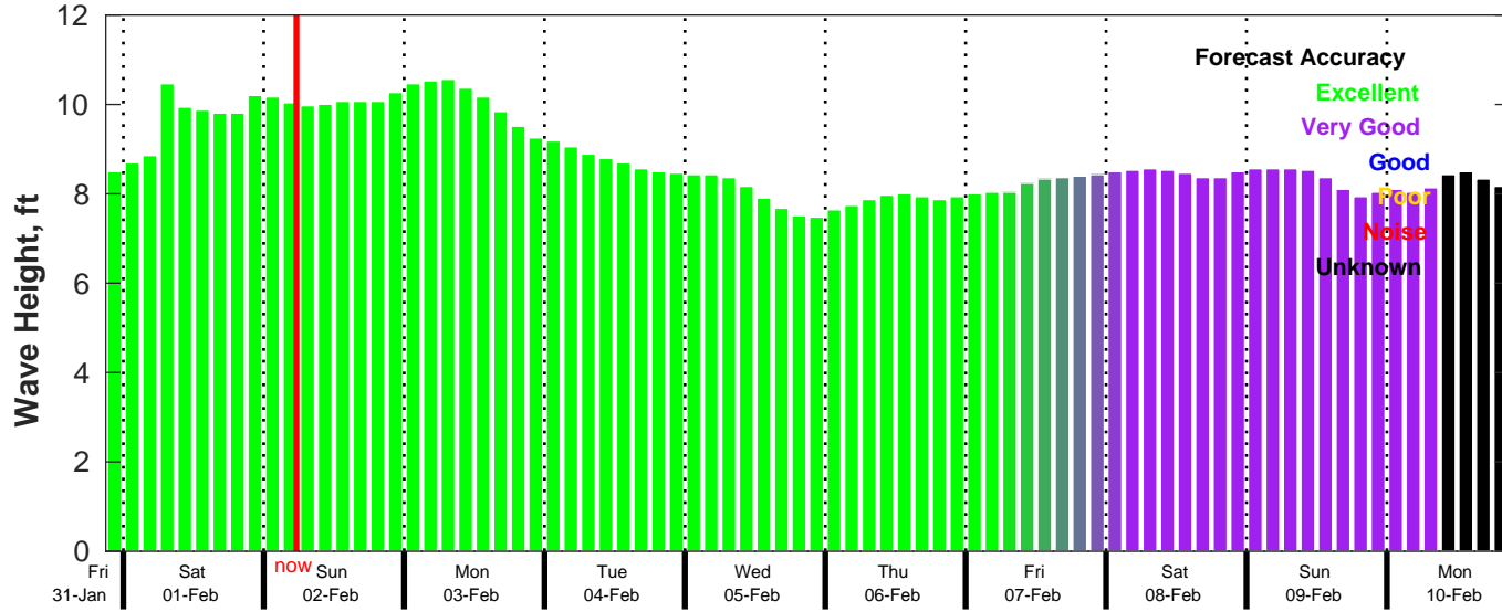
CMEMS Wave Forecast for NDBC 41040 from 31-Jan-2025 21:00:00 to 10-Feb-2025 21:00:00
