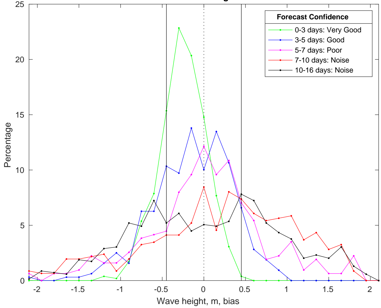
NDBC 42019 vs GFSWaves Bias Histogram: 02-Feb-2025
