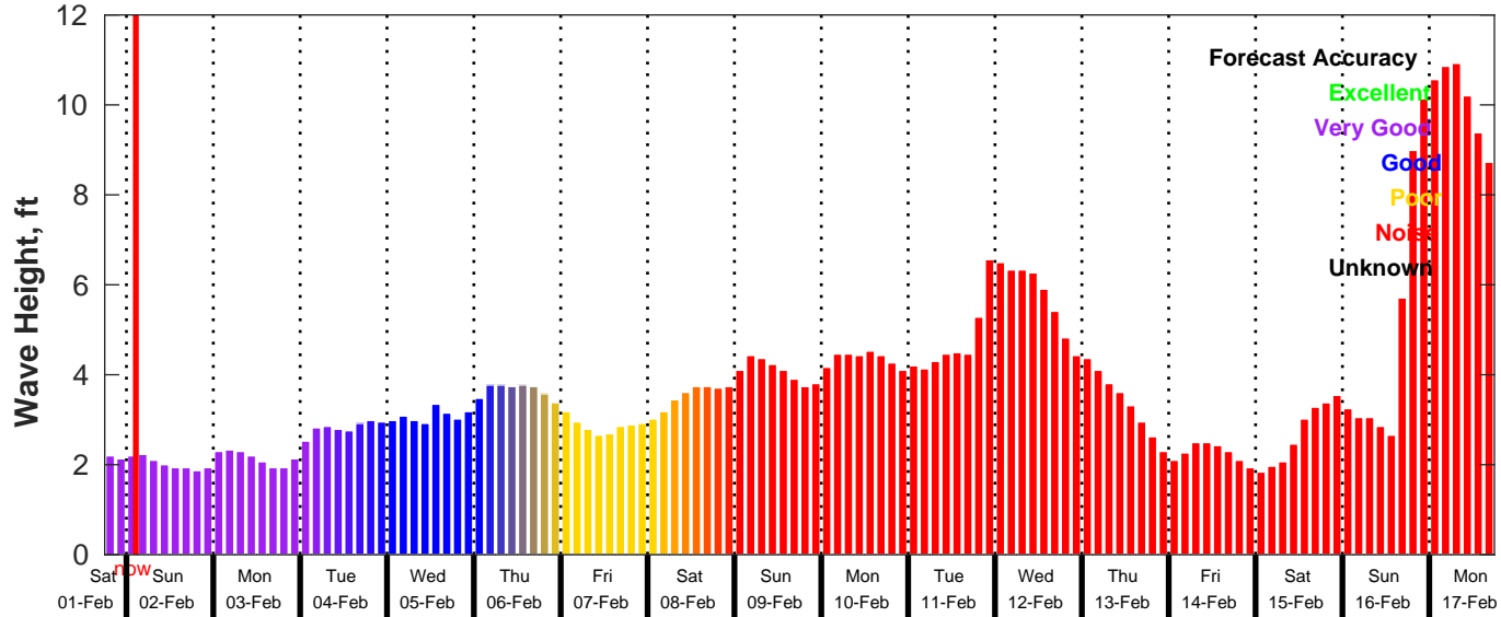
GFS Wave Forecast for NDBC 42019 from 01-Feb-2025 18:00:00 to 17-Feb-2025 18:00:00
