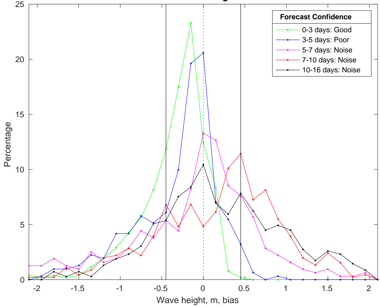
NDBC 42020 vs GFSWaves Bias Histogram: 02-Feb-2025
