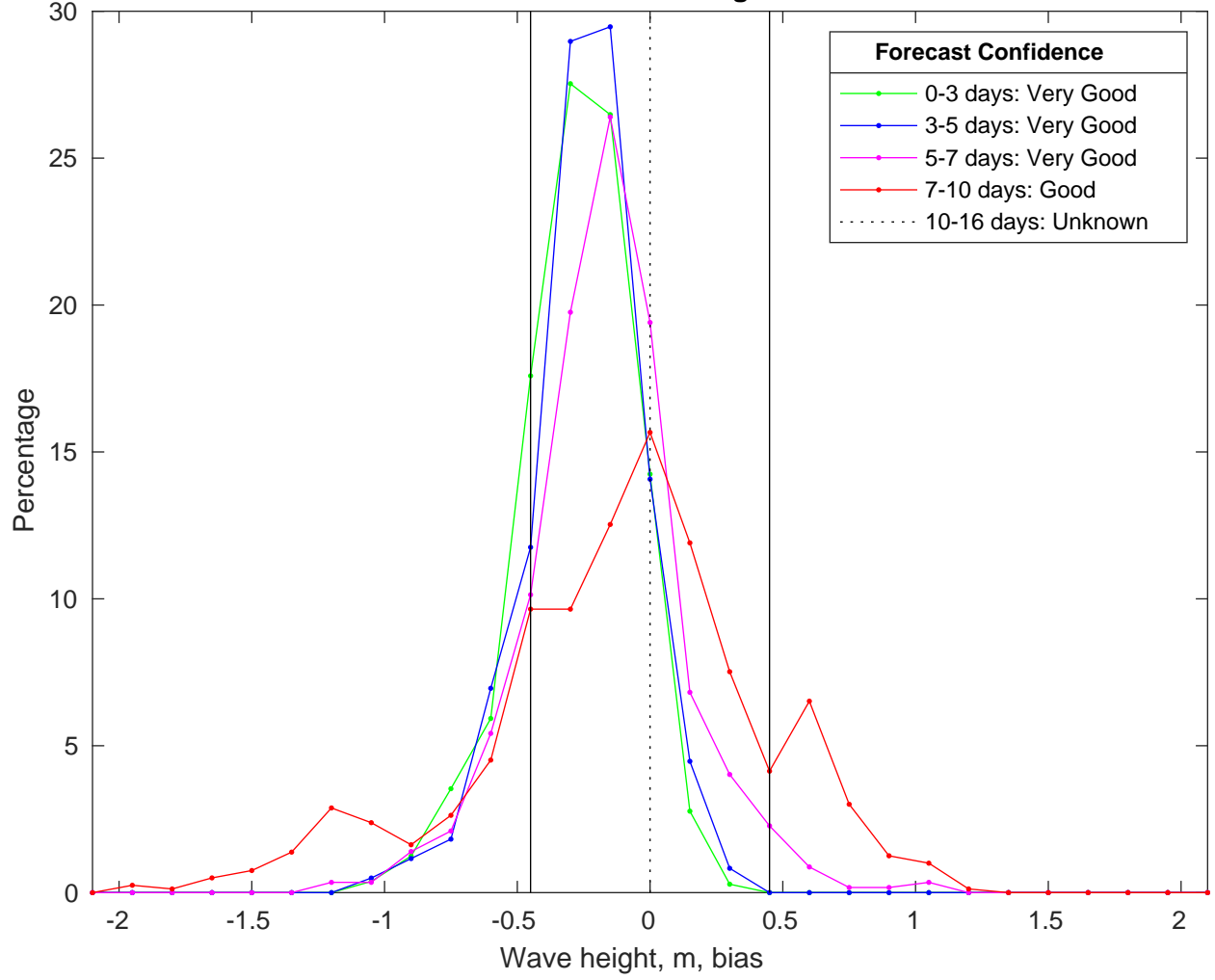
NDBC 42035 vs CMEMSWaves Bias Histogram: 02-Feb-2025
